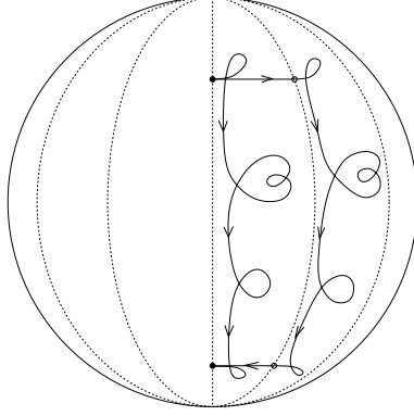
FIGURE 3. Approximating a curve by a locally convex curve
