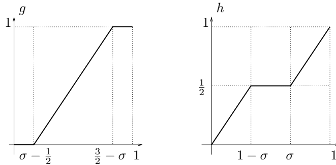
FIGURE 4. The functions g_\sigma and h_\sigma
