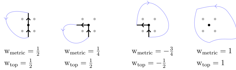
Figure 11: Illustration of topological and metric weights. The points in \mathcal{N}_v are in grey.
