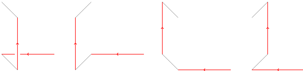
Figure 13: Illustrations of the four different projections \Pi_{\pm\epsilon, \pm\epsilon}^\beta of two segments \ell_0, \ell_1 with \tau^{\vec{\beta}_3}(\ell_0, \ell_1) = 1/4 . The dotted lines represent the projection of lines which are parallel to \vec{\beta}_3 , in each of the four cases. Notice that the segments are involved in a crossing for exactly one of the projections, and this crossing is positive.
