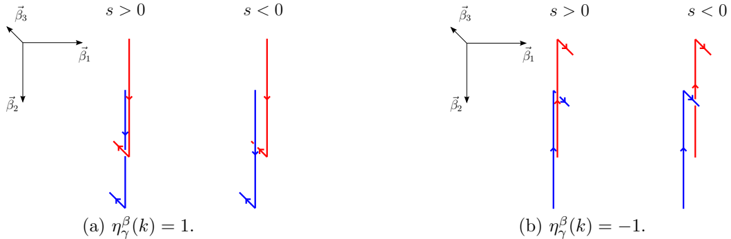
Figure 14: Illustration of the crossings \Pi_{\epsilon, \epsilon}^\beta(\gamma) \cap \Pi_{\epsilon, \epsilon}^\beta(\gamma + s\vec{\beta}_1 + b\vec{\beta}_2 + c\vec{\beta}_3) for s \in [-a, a] . Notice that simultaneously switching the orientations of both segments does not change the signs of the crossings.
