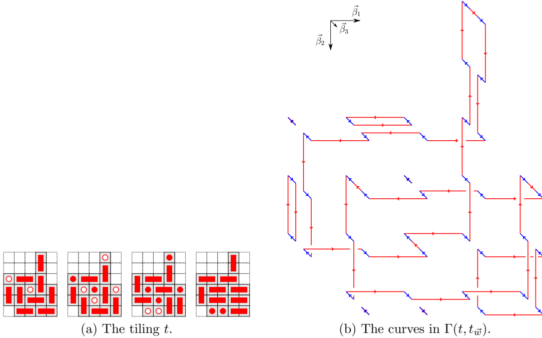
Figure 15: A tiling t of a \vec{w} -multiplex with depth 4, and \Gamma(t, t_{\vec{w}}) , where t_{\vec{w}} is the tiling such that every dimer is parallel to \vec{w} . The dimers of t are the red segments, and the blue segments are the ones in (-t_{\vec{w}}) . We chose a basis \beta \in \mathbf{B} with \vec{w} = \vec{\beta}_3 ; \vec{w} points “towards the paper”. \Gamma(t, t_{\vec{w}}) consists of nine curves, four of which are trivial; the five nontrivial curves form \Gamma^*(t, t_{\vec{w}}) .
