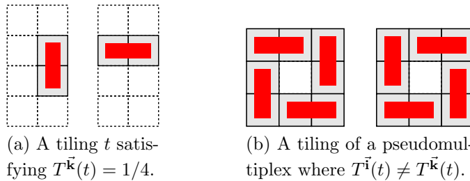
Figure 19: Two examples of tilings: \vec{k} is chosen to point towards the paper.
