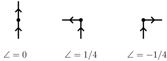
Figure 12: Illustration of the angle of a vertex.
