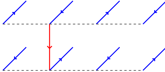
Figure 16: A dimer \ell_0 parallel to \vec{w} , portrayed in red, and the pairs of segments (blue) of t_{\vec{k}} affected by it: \vec{u} -effects cancel.
