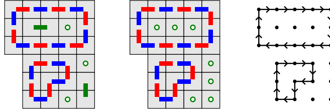
Figure 10: A tiling with two trivial cycles; the same tiling with the two trivial cycles flipped into jewels; and the sock that corresponds to both of them.
