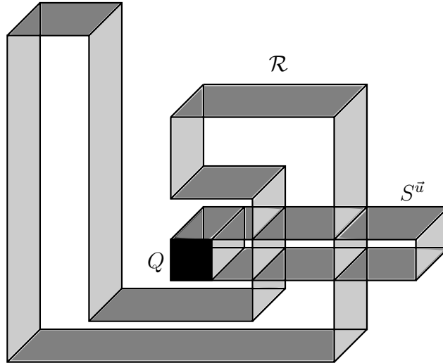
Figure 17: A multiplex \mathcal{R} with base \mathcal{D} \subset \pi and depth N , a basic square Q \subset \pi , Q \notin \mathcal{D} and the shade \mathcal{S}^{\vec{u}}(Q + [0, N]\vec{w}) .
