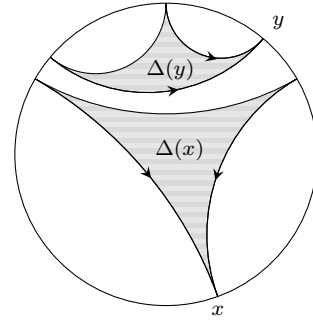
FIG. 5. x \neq y \in N_1^\perp ; the triangles \Delta(x) and \Delta(y) have disjoint interiors.
