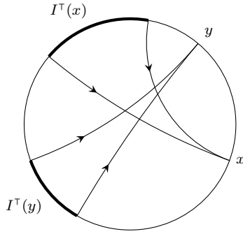
FIG. 4. x \neq y \in N_1^\top ; the intervals I^\top(x) and I^\top(y) have disjoint interiors.
