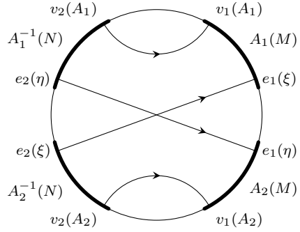
FIG. 8. An example with K^\perp = \{1^\infty, 2^\infty\} .
