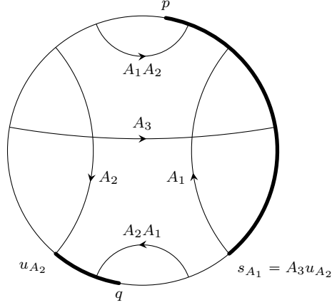
FIG. 6. The example of Proposition A.2. The thick part represents the “non-strict multicone” M . For each L , the arrow labelled L represents the hyperbolic geodesic from s_L to u_L .
