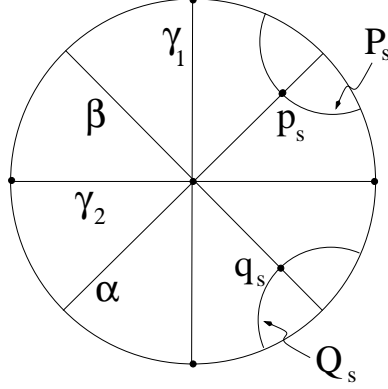
FIGURE 6. w = \gamma_1 \cap \gamma_2 = 0 .
