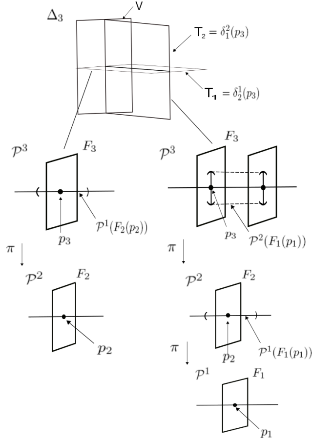
FIGURE 3. Critical hyperplane configuration over p_3 \in RVL .
