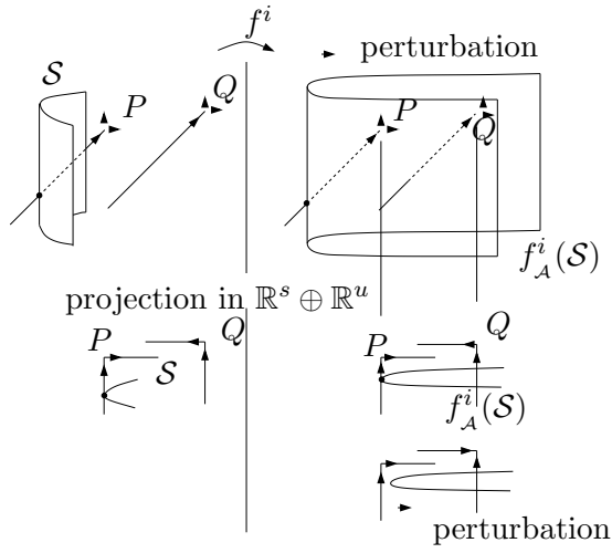
Figure 6: Folded manifold: case (b).
