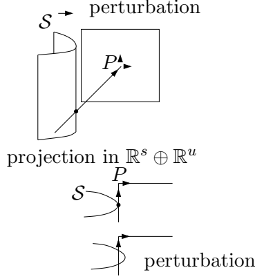
Figure 5: Folded manifold: case (a).
