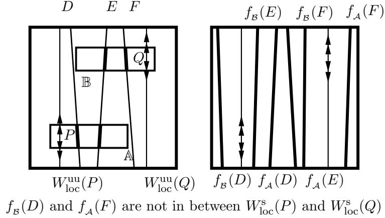
Figure 4: Projection in \mathbb{R} \oplus \mathbb{R}^u . Disks in between W_{\text{loc}}^s(P) and W_{\text{loc}}^s(Q) and their images.
