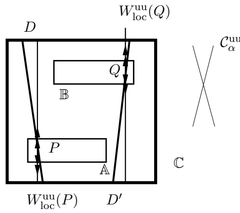
Figure 3: Projection in \mathbb{R} \oplus \mathbb{R}^u . uu-disks. Condition BH4 ).
