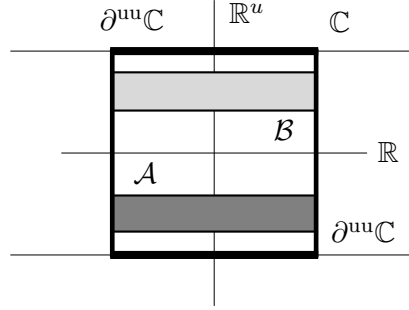
Figure 1: Projection in \mathbb{R} \oplus \mathbb{R}^u of a blender horseshoe. Condition BH1) .
