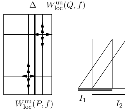
Figure 9: uu-disks and one-dimensional reduction.
