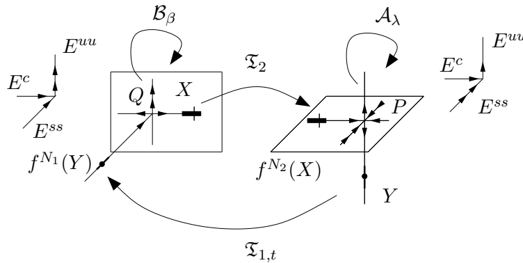
Figure 10: The model maps F_{\lambda,\beta,t}^{\pm,\pm} .
