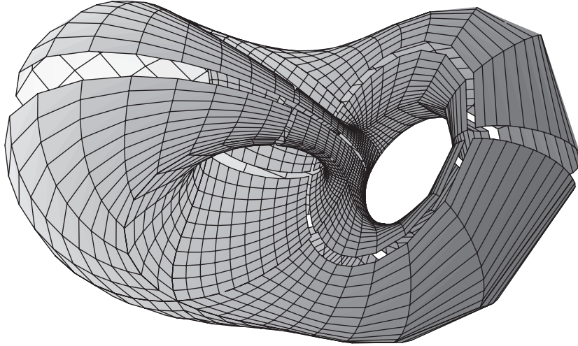
Figure 1: The cell decomposition of \mathcal{T}_\Lambda for \Lambda = \text{diag}(4, 5, 7)
