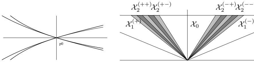
Figure 2: The set \mathcal{X}
