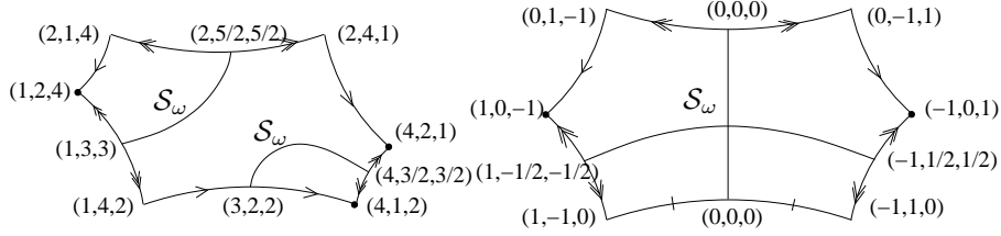
Figure 3: The phase space of Wilkinson's step for n = 3 .
