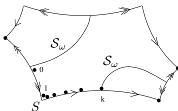
Figure 4: We may have F_\omega^k(T) \in \mathcal{S}_\omega for large values of k .
